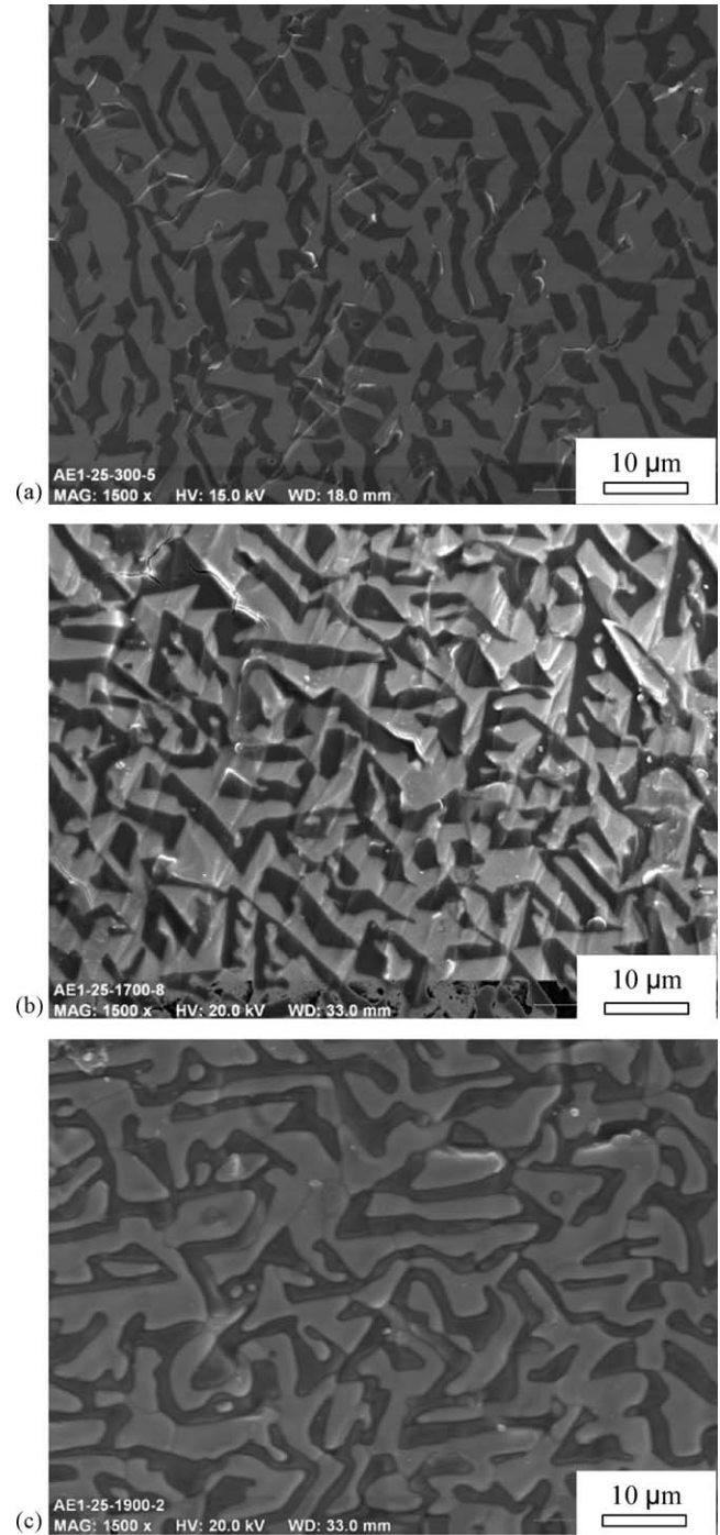
Fig. 11. Fracture surfaces of \text{Al}_2\text{O}_3\text{-Er}_3\text{Al}_5\text{O}_{12} eutectic rods grown at 25 mm/h tested at (a) 300 K, (b) 1700 K and (c) 1900 K.
