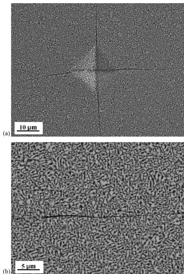
Fig. 6. (a) Cracking pattern and (b) crack propagation detail of the \text{Al}_2\text{O}_3 - \text{Er}_3\text{Al}_5\text{O}_{12} eutectic rod grown at 750 mm/h under an indentation load of 4.9 N.
