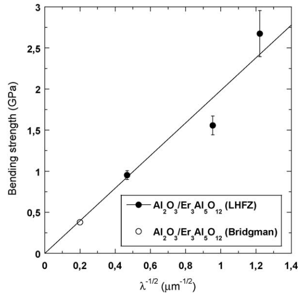
Fig. 8. Bending strength of \text{Al}_2\text{O}_3\text{--Er}_3\text{Al}_5\text{O}_{12} eutectic rods grown by the LHFZ method as a function of lamellar spacing. The experimental result Waku et al. 39 for rods grown using the Bridgman method is also included. The line corresponds to the predictions of Eq. (3) with K_{IC} = 2.3 \text{ MPa m}^{1/2} .
