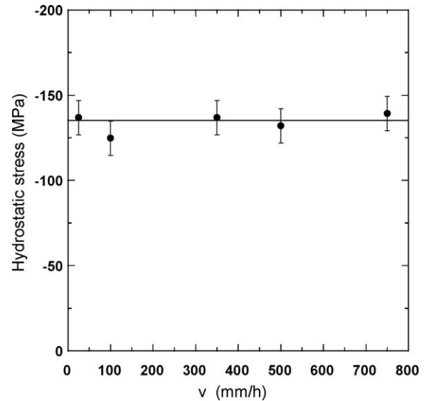
Fig. 4. Hydrostatic residual stresses in the \text{Al}_2\text{O}_3 phase measured on \text{Al}_2\text{O}_3\text{-Er}_3\text{Al}_5\text{O}_{12} eutectic rods as a function of the growth rate.
